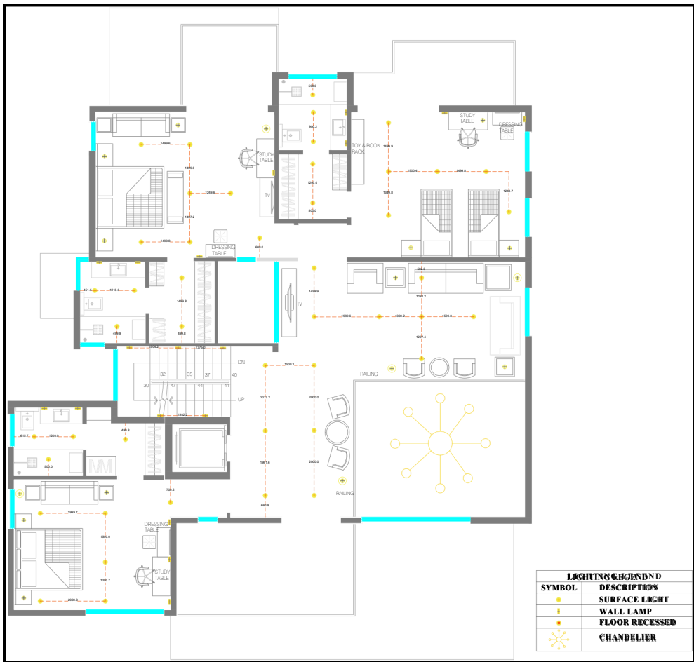
Lighting plan
