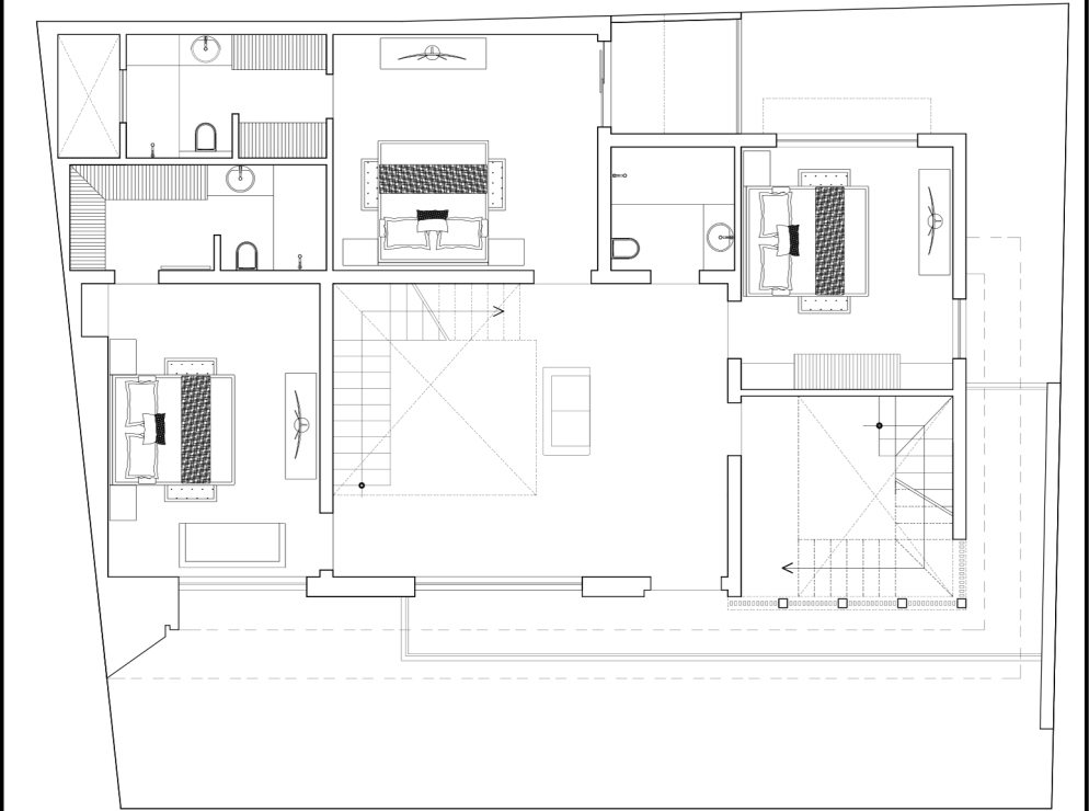
Floor Plans
